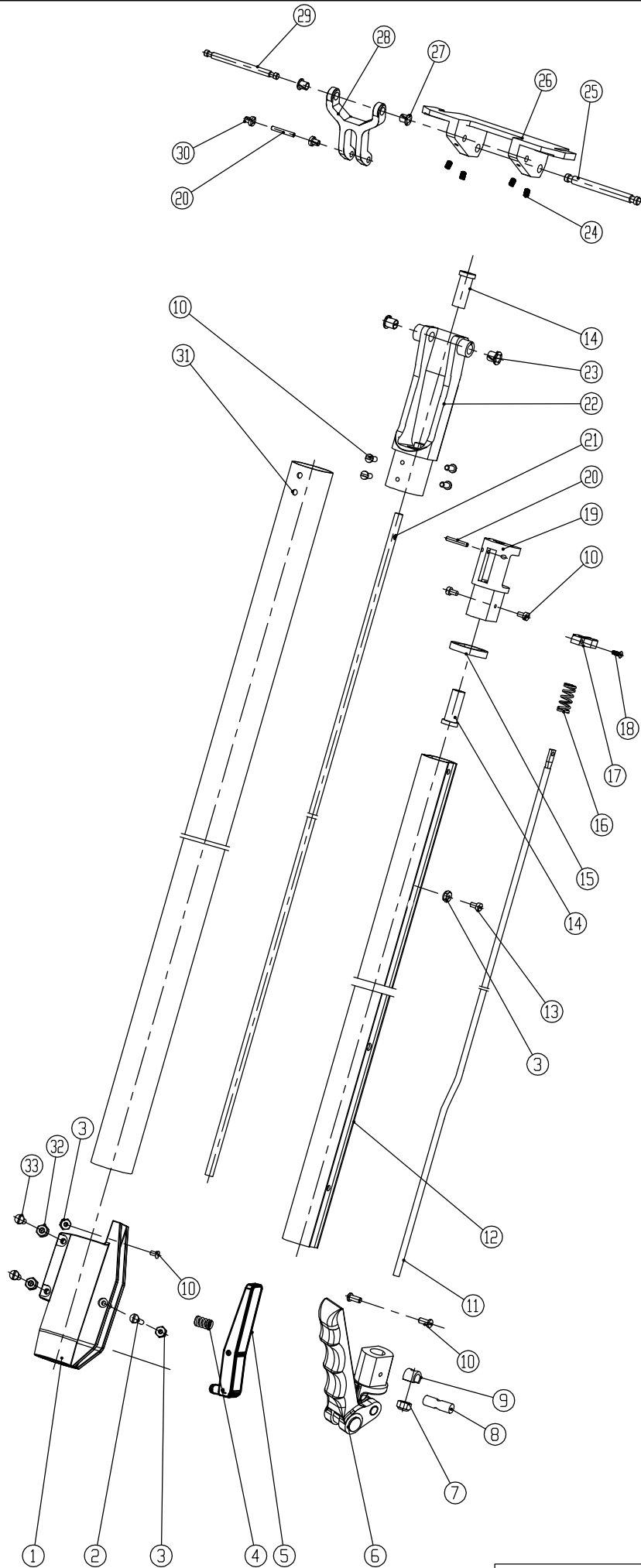
4-782 Ext Box Handle
